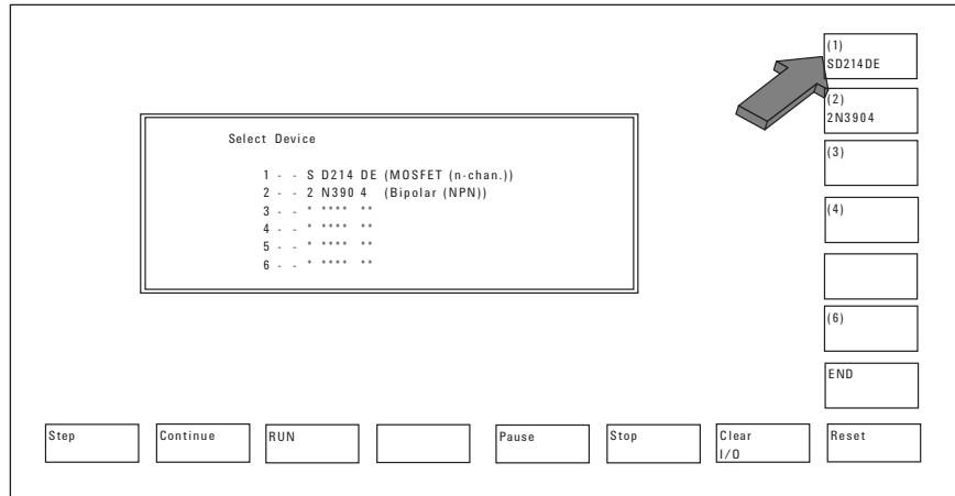
Figure 1. Example of a Test Device Selection Display
