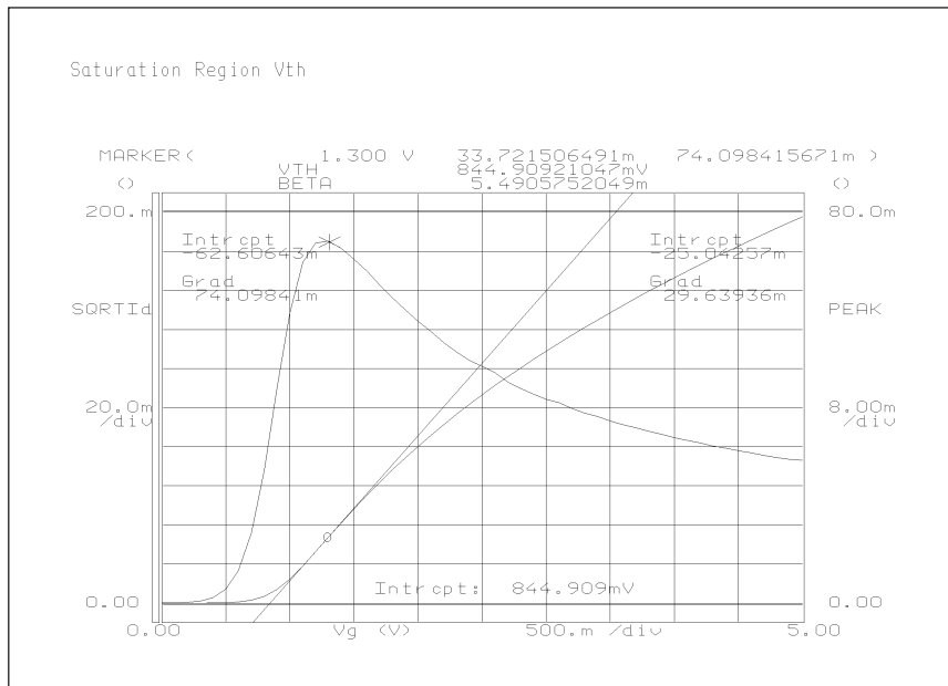
Figure 4. Example of Threshold Voltage Measurement
