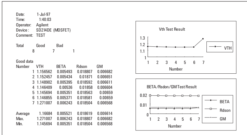
Figure 5. Example of Data Processed Using Microsoft Excel
